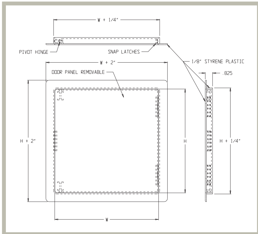
PA-3000 View of door back
